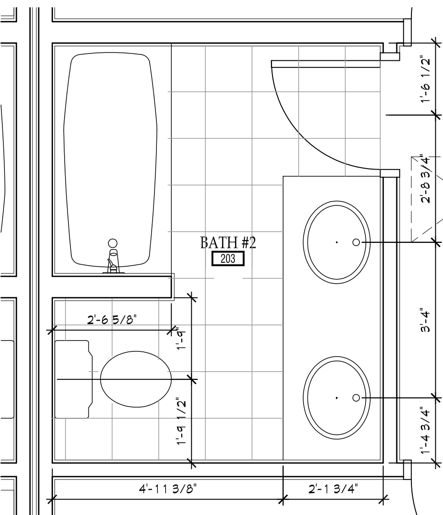
5 A200 ENLARGED BATHROOM PLAN 1/2" = 1'-0"
