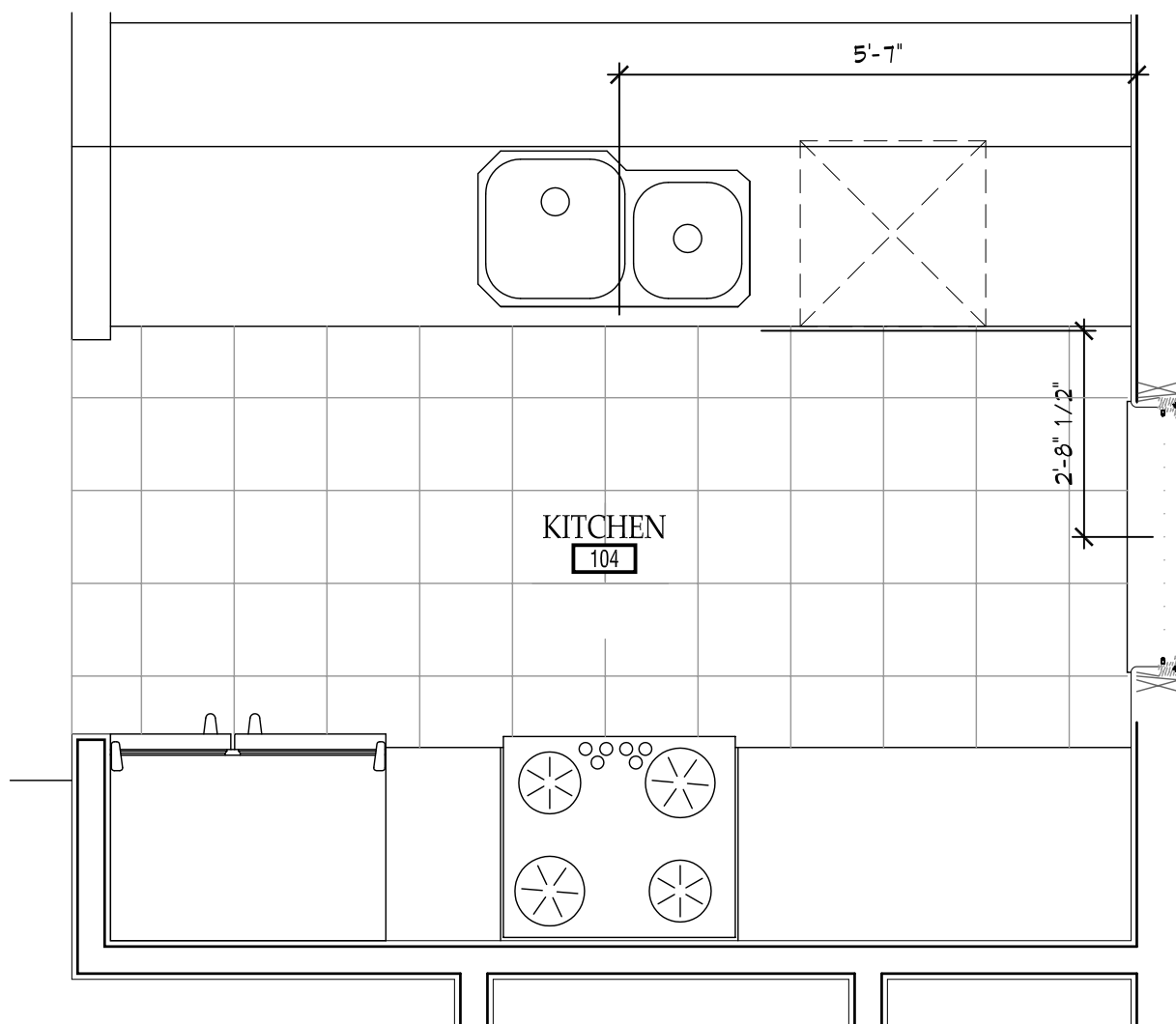
4 A200 ENLARGE KITCHEN PLAN 1/2" = 1'-0"
