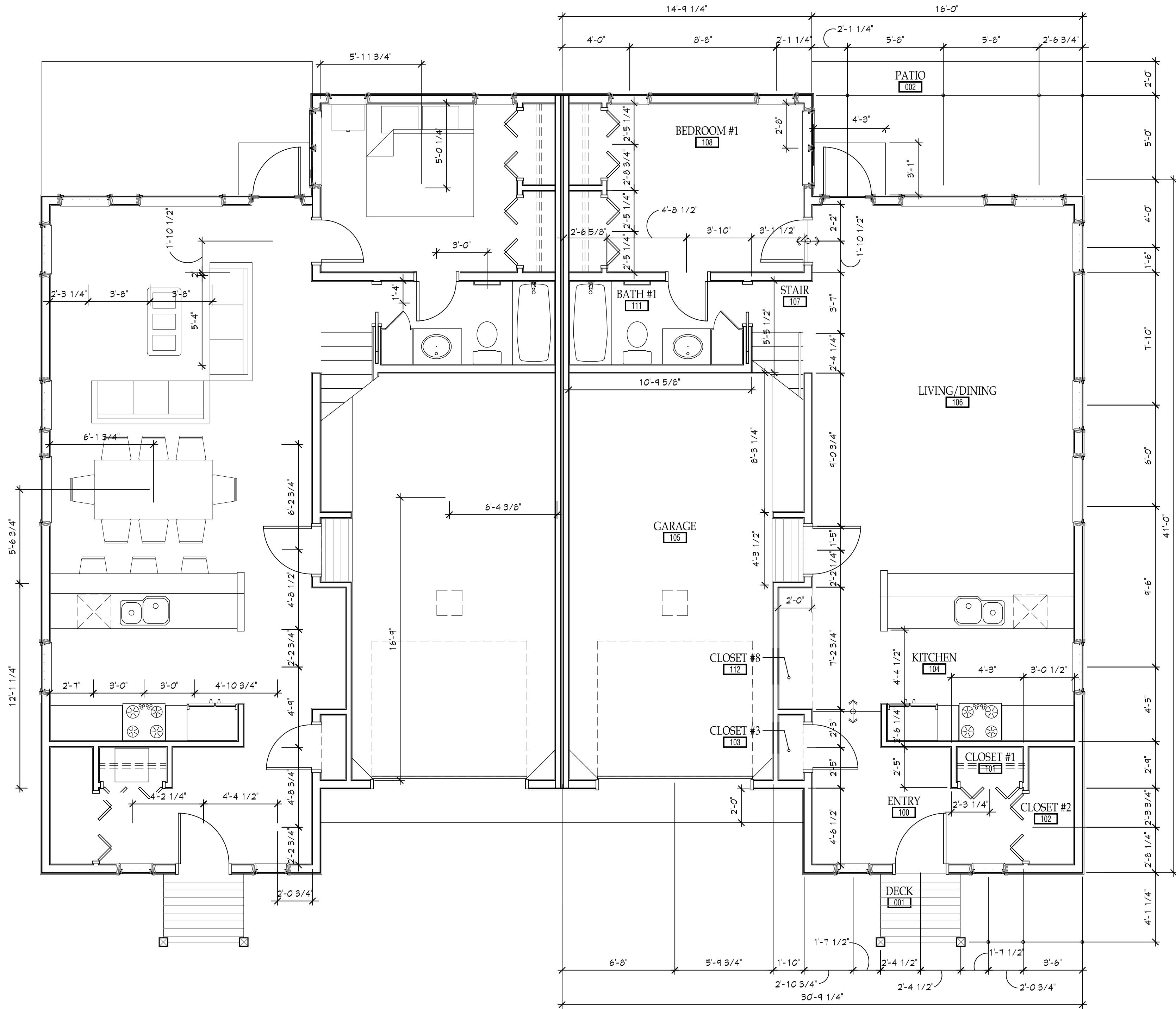
1 A200 FIRST FLOOR ELEC/ARCH PLANS 1/4" = 1'-0"
