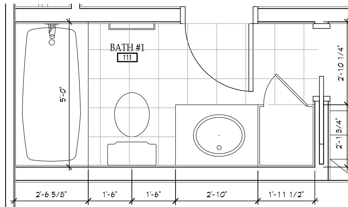
3 A200 ENLARGED BATHROOM PLAN 1/2" = 1'-0"
