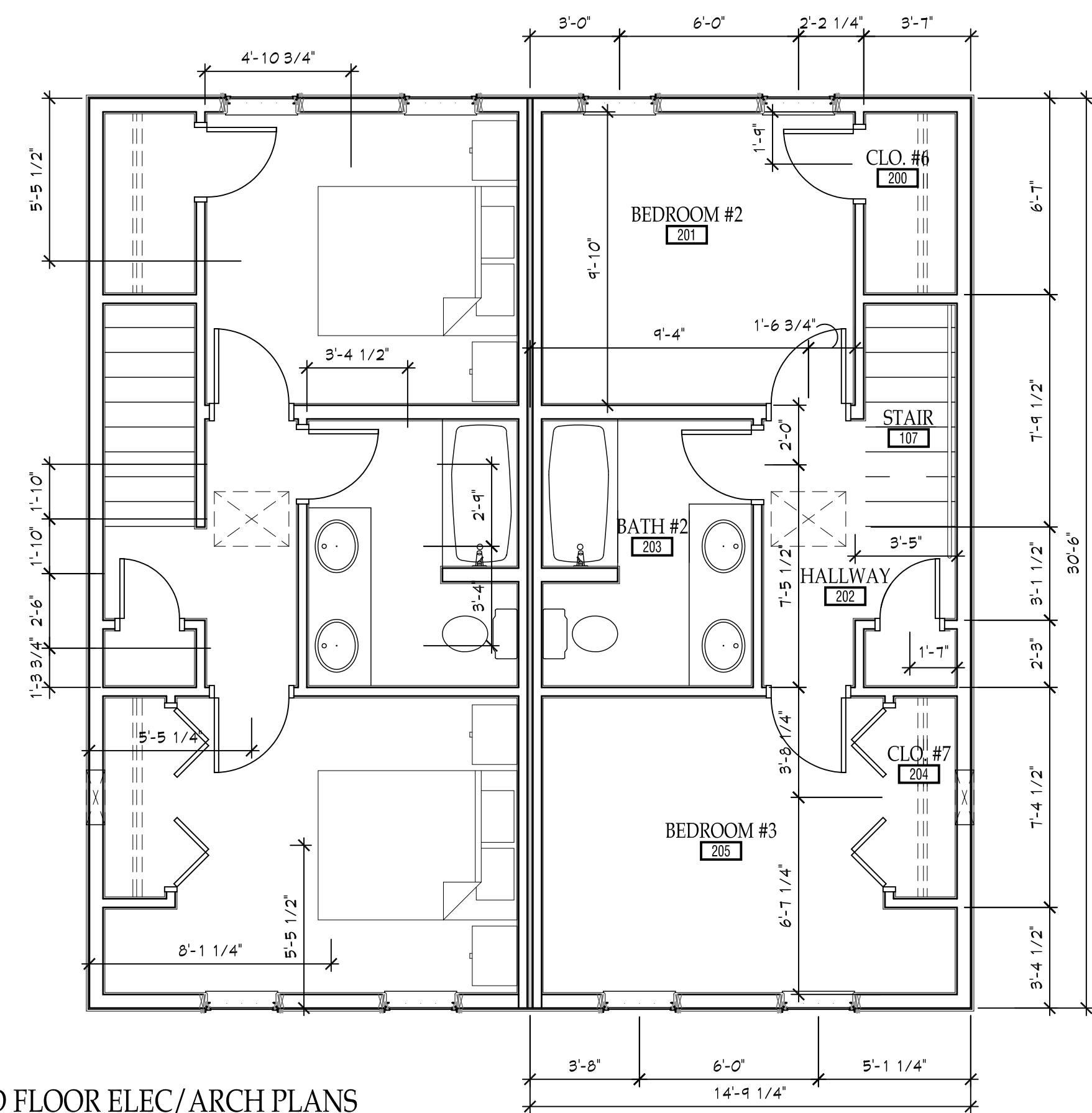
2 A200 SECOND FLOOR ELEC/ARCH PLANS 1/4" = 1'-0"
